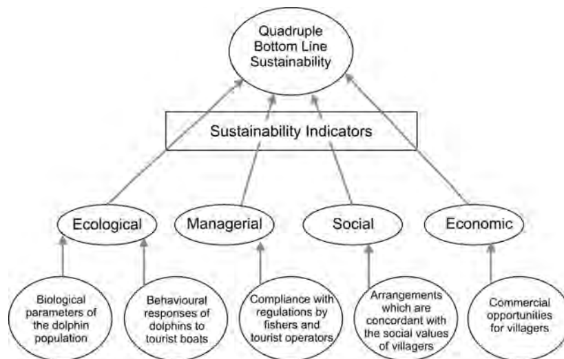
FIGURE 15.6 Conceptual framework for the arrangements required to ensure the sustainability of the Mekong River dolphin population. Modified from a diagram developed by Alastair Birtles and his research group at James Cook University.
