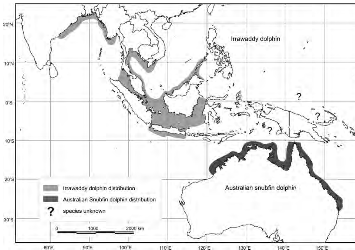
FIGURE 15.3 Distribution map of the Irrawaddy and Australian Snubfin dolphin.
