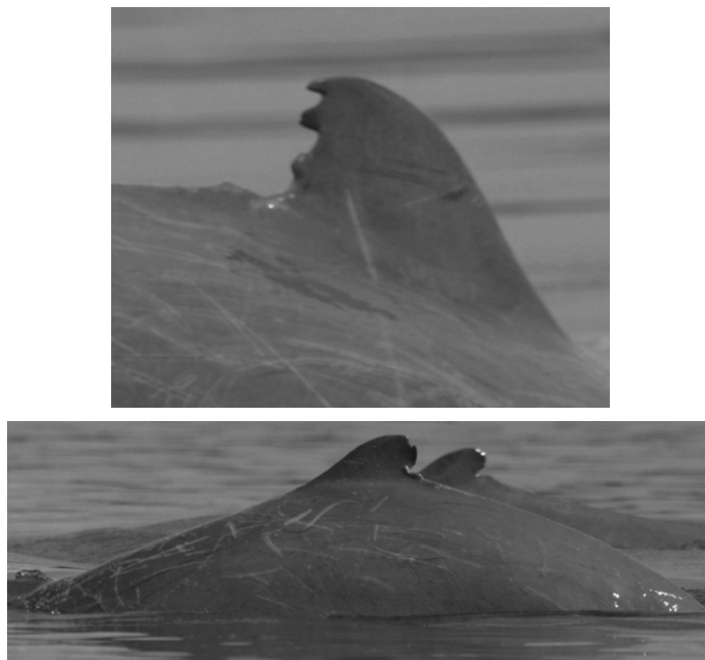
FIGURE 15.5 Photo-identification was one of the primary techniques used to estimate abundance of Irrawaddy dolphins in the Mekong River. Examples of excellent quality photographs of two well-known dolphins; KA05 Rags (top) and CH01 Chital (bottom), used in the capture-recapture analysis.
